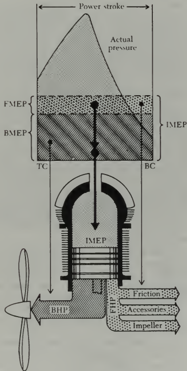
FIGURE 1-30. Powers and pressures.
